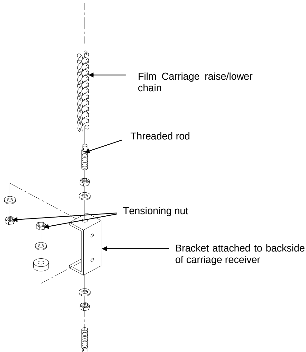
Figure 7B: Film Carriage Lift Chain Adjustment
