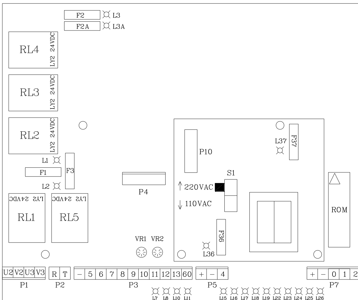
Figure 4: Microprocessor Card for the Predator SS
